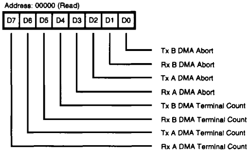
Figure 12. DMA Status Register
