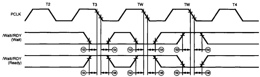
Figure 48. Wait and Ready Timing
