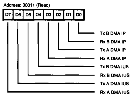
Figure 16. Interrupt Status Register
