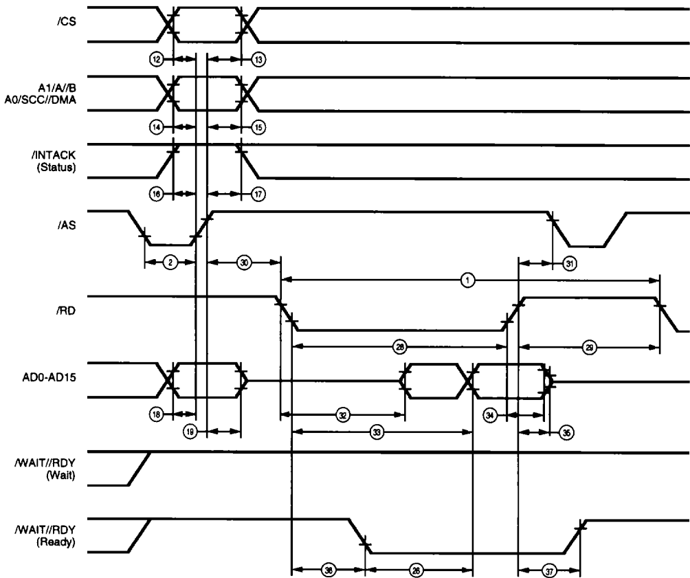
Figure 30. Multiplexed /RD Read Cycle
