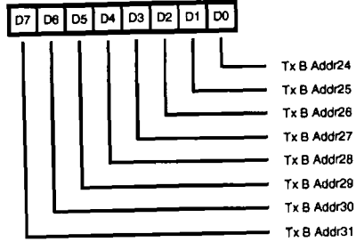
Figure 26. Transmit DMA Address Register Channel B
