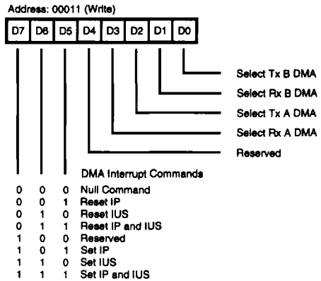
Figure 15. Interrupt Command/Register
