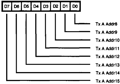
Figure 24. Transmit DMA Address Register Channel A
