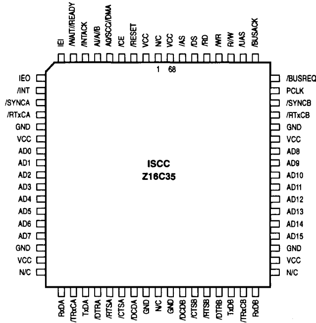
Figure 2. Pin Assignments
