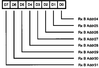
Figure 25. Receive DMA Address Register Channel B
