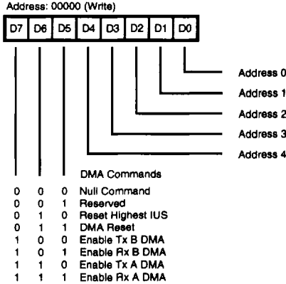
Figure 11. Channel Command/Address Register
