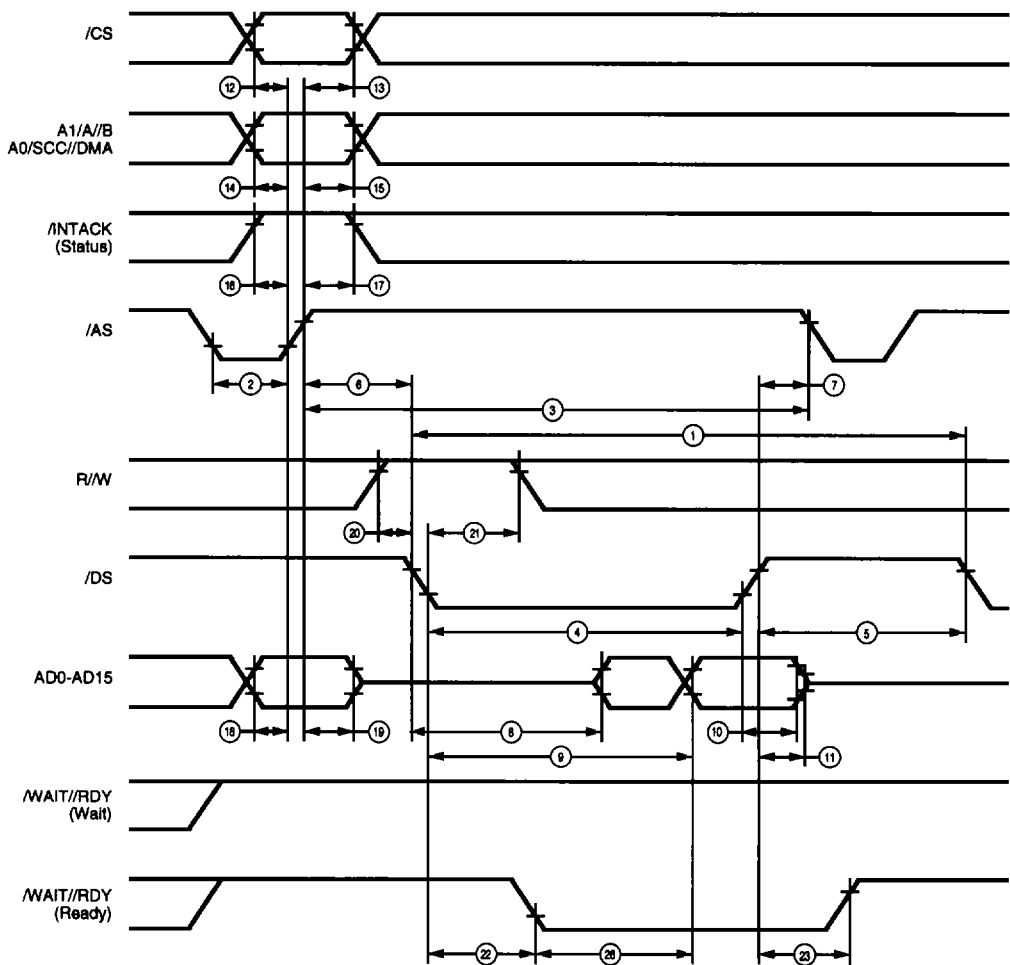
Figure 28. Multiplexed /DS Read Cycle
