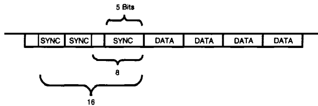
Figure 5. Detecting 5- or 7-Bit Synchronous Characters
