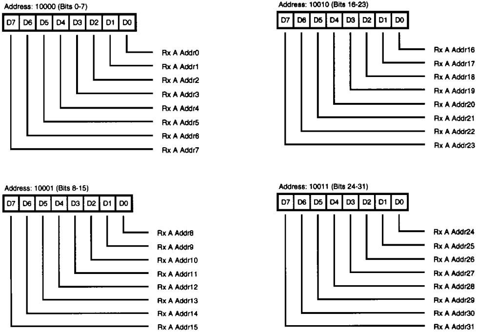
Figure 23. Receive DMA Address Register Channel A
