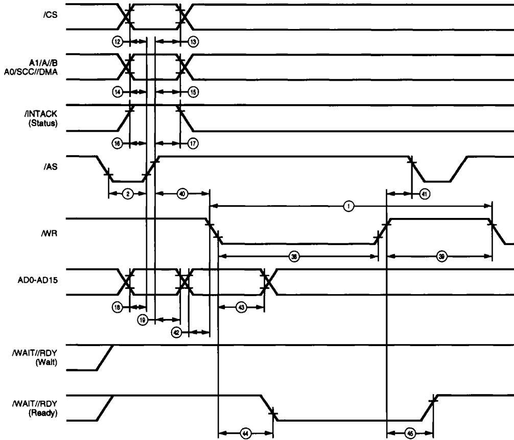
Figure 31. Multiplexed /WR Write Cycle
