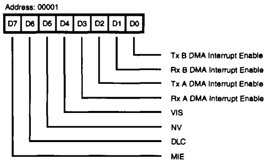
Figure 13. Interrupt Control Register
