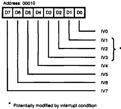
Figure 14. Interrupt Vector Register
