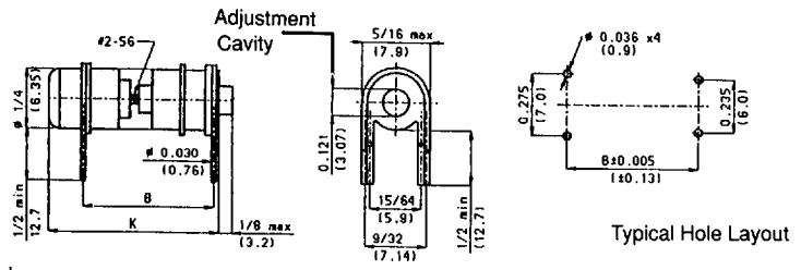
Fig. 5 Printed Circuit 4 Wire Series
