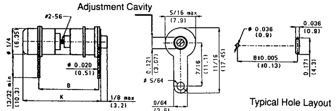
Fig. 6 Printed Circuit Lug and Lead Series
