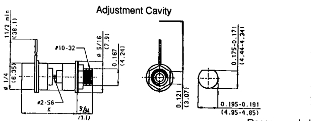
Fig. 4 Panel Mount Series
