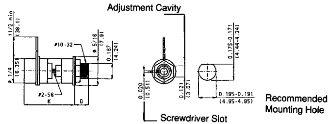
Fig. 1 Panel Mount Series
