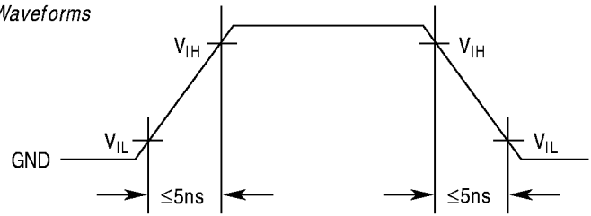
Input Waveforms
