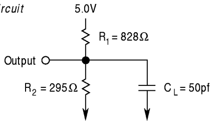
Load Circuit
