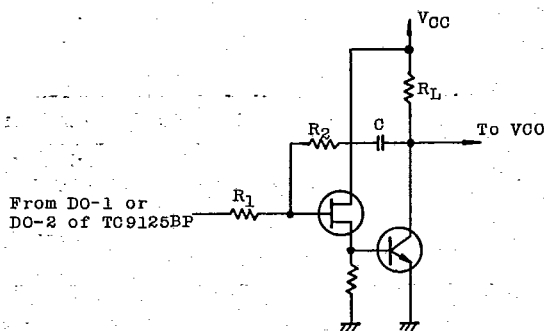
FIG. 10 LOW PASS FILTER CIRCUIT
