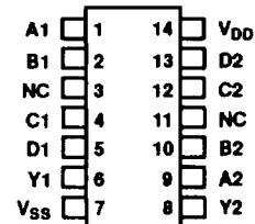
14-Pin DIP Top View
